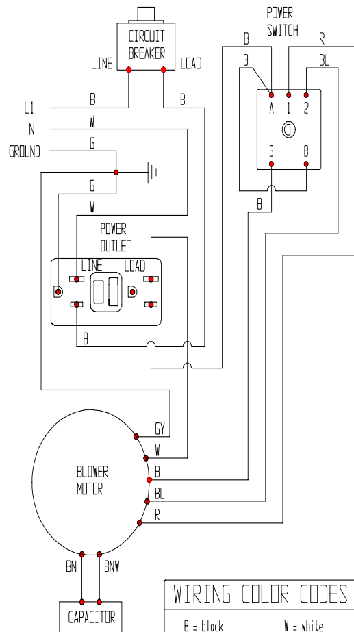
SAHARA PRO X3 - 115V 60HZ WIRING DIAGRAM
